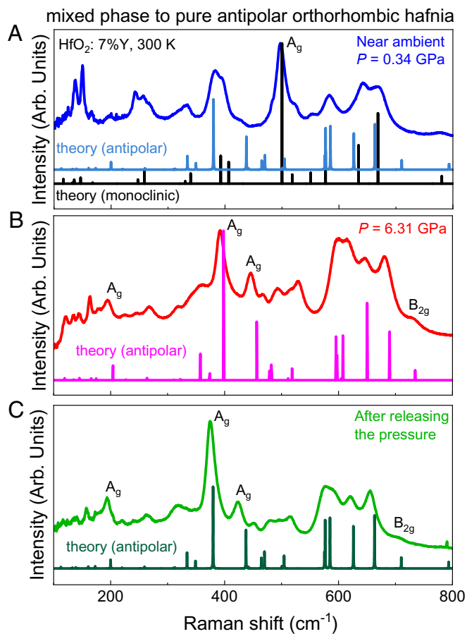
Fig. 2. (A) Raman scattering response of \text{HfO}_2:7\%Y at room temperature in a closed diamond anvil cell. This sample consists of mixed monoclinic + antipolar orthorhombic structures at 0.34 GPa. Theoretically calculated Raman spectra of the pure monoclinic ( P2_1/c ) and antipolar orthorhombic ( Pbca ) phases at zero pressure are plotted below the experimental data. (B) Raman scattering response of \text{HfO}_2:7\%Y at room temperature and P = 6.3 GPa. The theoretical Raman spectrum of the antipolar orthorhombic ( Pbca ) phase of hafnia at the same pressure is included below. (C) Raman scattering response of \text{HfO}_2:7\%Y at room temperature after release. As discussed in the main text, a pure antipolar orthorhombic ( Pbca ) phase appears above 6.3 GPa which is trapped upon release of the pressure. The theoretical Raman spectrum at zero pressure is included as well. The symmetries of the signature modes are labeled for each phase (34). Note that there is additional symmetry breaking occurring in the experimental data due to Y stabilizer incorporation (34).
