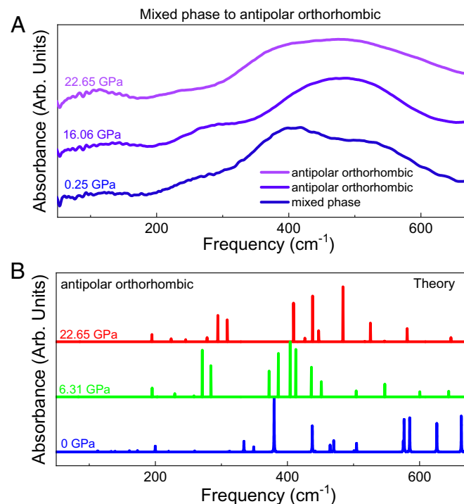
Fig. 3. (A) Synchrotron-based infrared absorbance of mixed-phase \text{HfO}_2:7\%Y as a function of pressure. The antipolar orthorhombic ( Pbca ) phase is formed under compression. Pressures up to 22.65 GPa do not yield the polar orthorhombic phase—at least not in a straightforward manner at room temperature. We also do not see evidence for the cotunnite phases (28), probably due to the presence of Y stabilizer. The spectra are offset for clarity. (B) Calculated mode patterns of antipolar orthorhombic ( Pbca ) hafnia at different pressures for comparison.
