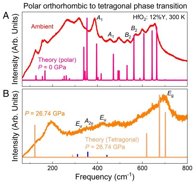
Fig. 4. (A) Raman scattering response of \text{HfO}_2:12\%Y at ambient conditions compared with the results of our lattice dynamics calculations. The symmetries of the signature modes for polar orthorhombic hafnia are labeled. (B) Compression drives a transition from the polar orthorhombic ( Pca2_1 ) to the tetragonal ( P4_2/nmc ) phase. The theoretically calculated Raman spectrum of tetragonal hafnia is shown for comparison. In addition to the fundamental excitations of the lattice associated with each phase, there is evidence for additional features (shown in blue) that we assign as infrared-active modes appearing due to symmetry breaking induced by Y substitution (34). Based upon the peak shapes, the sample is still in single crystal form at 26.74 GPa.
