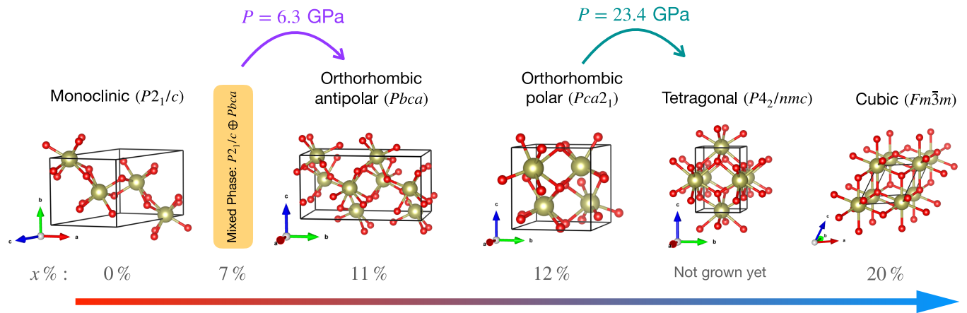
Fig. 1. Summary of the various phases of hafnia of interest in this work, i.e., monoclinic HfO 2 (the ground state), and the higher-energy metastable phases arranged in the order of their increasing formation energy. When formed by laser floating zone + rapid cooling techniques (20), Y concentrations of 0, 7, 11, 12, and 20% yield monoclinic, mixed monoclinic and antipolar orthorhombic, antipolar orthorhombic, polar orthorhombic, and cubic phases, respectively. A metastable tetragonal phase has been predicted from first principles but not yet realized by these growth methods. X-ray scattering as well as TEM studies of the initial products of this study are available in ref. 20. The space groups are indicated above. The polar orthorhombic material is switchable (i.e., ferroelectric), whereas antipolar orthorhombic hafnia is not switchable (i.e., not antiferroelectric) (20). The curved arrows at the top indicate the pressure-induced transitions discussed in the text.
