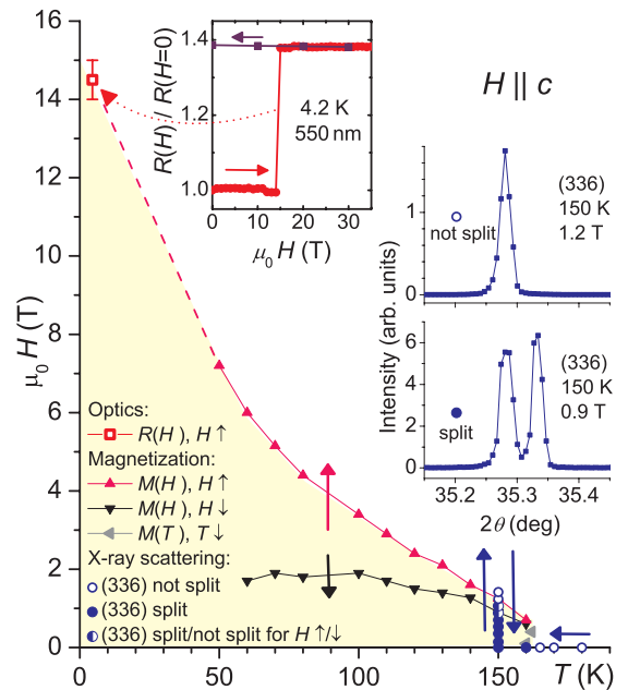
FIG. 3: (Color online) Low-temperature phase transition from magnetization data ( \blacktriangle , \blacktriangledown , see [9]), field-dependence of optical reflectance contrast R(H)/R(H = 0) at \lambda = 550 nm (squares, see left inset), and presence (indicated by \bullet ) or absence ( \circ ) of a splitting in the total diffraction angle of the structural Bragg reflection (336) from synchrotron x-ray scattering (right insets). The maximum region of the structurally distorted phase is shaded (see text).
