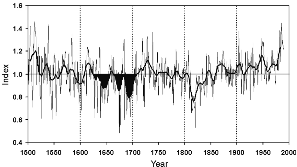
Figure 1. The standard tree-ring index chronology developed from 16 alpine chronologies in five central European countries (Grissino-Mayer et al. 2003 in press). The bold curve represents an 11yr moving average that accentuates the low-frequency trends. The Maunder Minimum is indicated in the shaded region between ca. AD 1620–1715.
