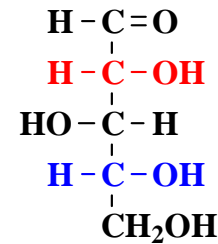
D-Xylose
