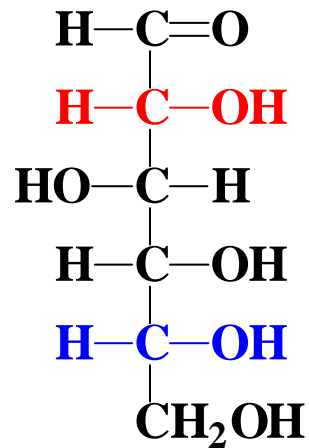
D-Glucose
