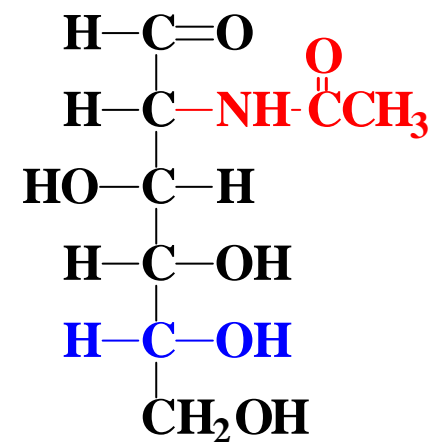
N-Acetyl- D-glucosamine
