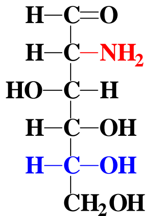
D-Glucosamine
