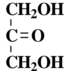
Dihydroxyacetone
