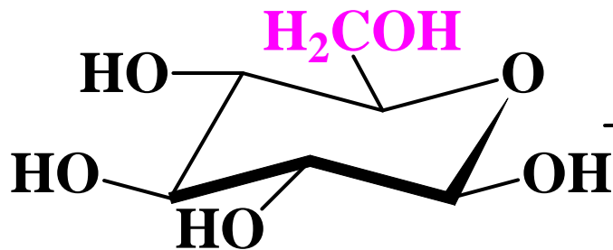
\beta -D-Glucose
