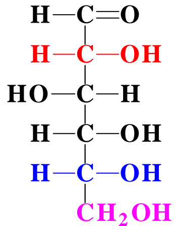
D-Glucose
