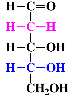
2-Deoxy-D-ribose
