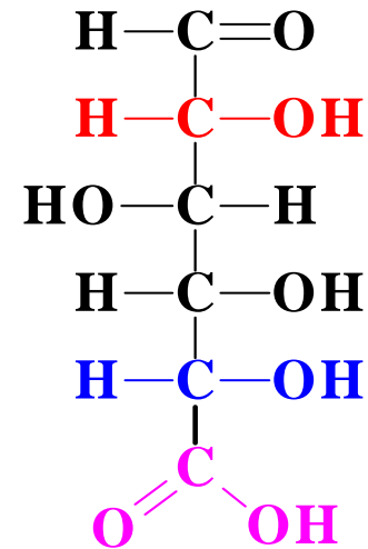
D-Glucuronic Acid
