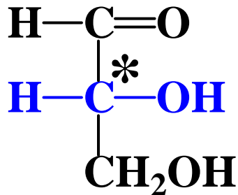
D-Glyceraldehyde
