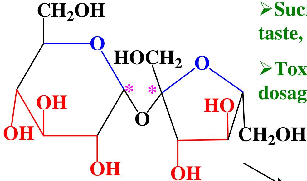
Sucrose
