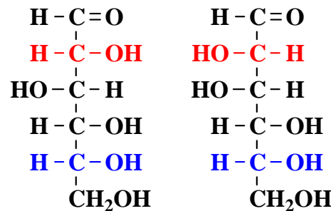
D-Glucose
